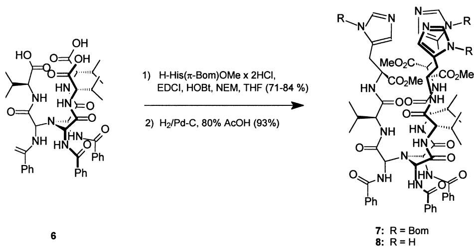
Scheme 1. Synthesis of the tripodal histidine ligand 8.
