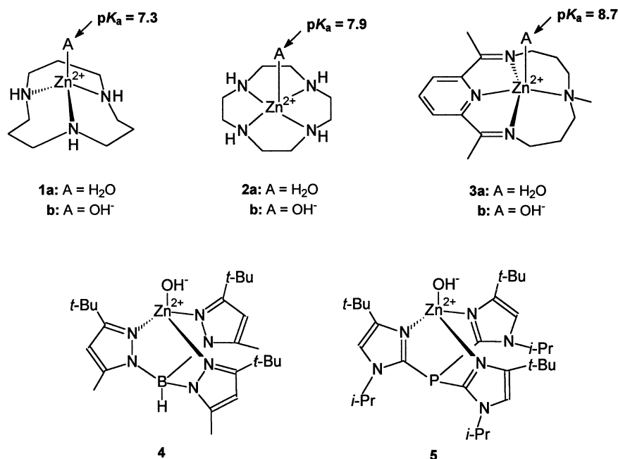
Figure 2. Mononuclear model complexes for carbonic anhydrase.
