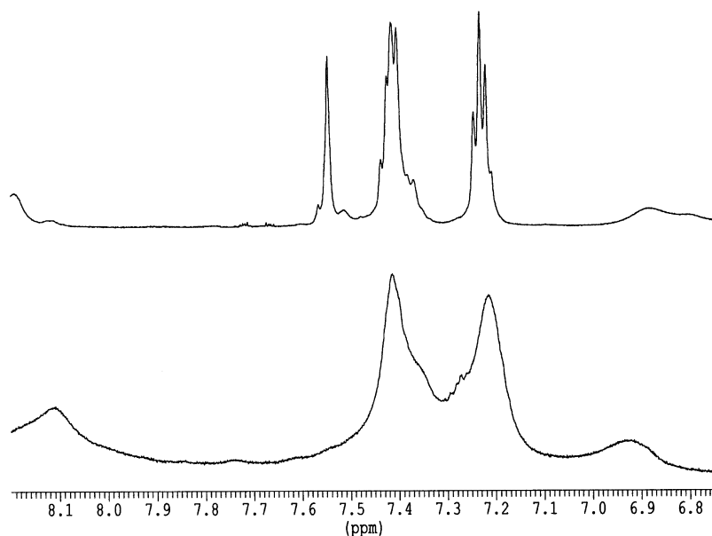
Figure 4. Aromatic region of the 600 MHz 1 H NMR spectra (DMSO- d 6 ) of histidine ligand 11 and its zinc(II) complex 13 .
