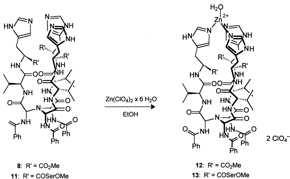
Scheme 3. Preparation of the zinc(II) complexes 12 and 13.
