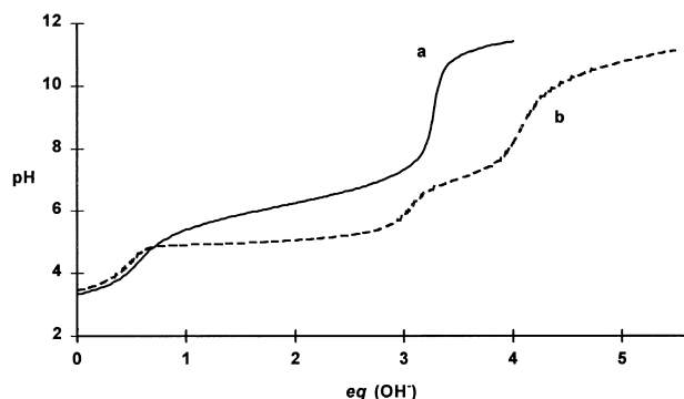
Figure 5. pH-Titration curves for N(BzGly*ValHisOMe) 3 ( 8 ) at I=0.10 (NaClO 4 ) and 25.0 °C in 33% EtOH: (a) 1.00 mM [L·3H + ] 3+ ; (b) solution a + 1.00 mM Zn 2+ SO 4 . eq(OH - ) is the moles of base (0.10 M NaOH) per mole of ligand.
