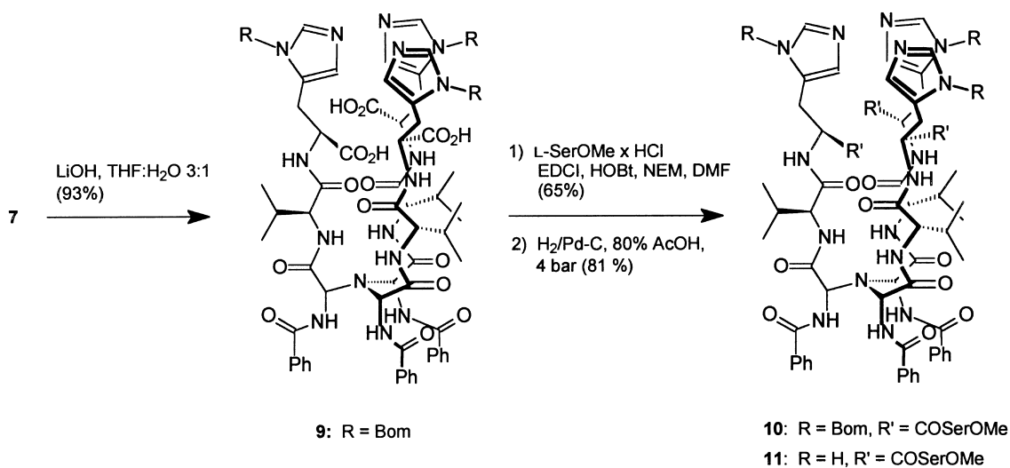
Scheme 2. Preparation of the tripodal histidine ligand 11.
