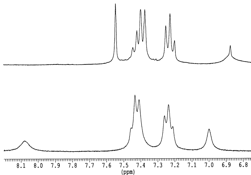
Figure 3. Aromatic region of the 300 MHz 1 H NMR spectra (DMSO- d 6 ) of histidine ligand 8 and its zinc(II) complex 12 .
