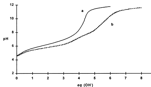
Figure 6. pH-Titration curves for N(BzGly*ValHisSerOMe) 3 ( 11 ) at I=0.10 (NaClO 4 ) and 25.0 °C in 52% EtOH: (a) 1.00 mM [L·3H + ] 3+ ; (b) solution a + 1.00 mM Zn 2+ SO 4 . eq(OH - ) is the moles of base (0.10 M NaOH) per mole of ligand.
