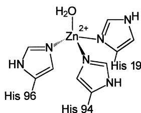
Figure 1. Active center of carbonic anhydrase.
